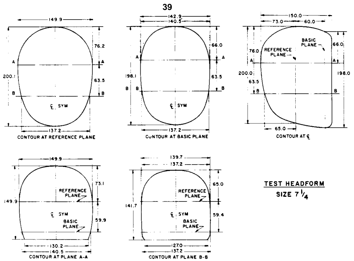
Figure 3. Test headform. Dimensions are in millimeters.
