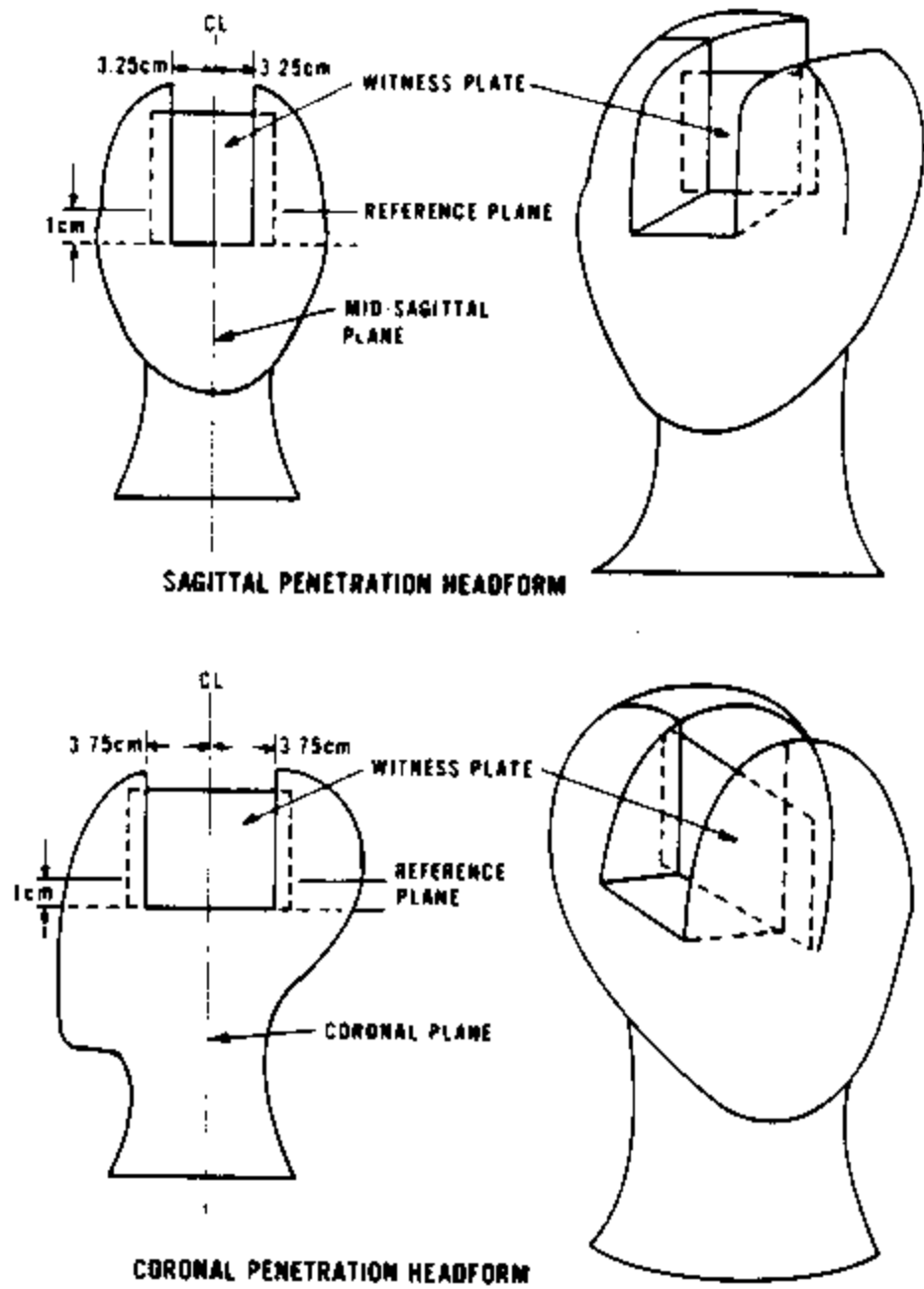
Figure 4. Ballistic penetration test headforms.
