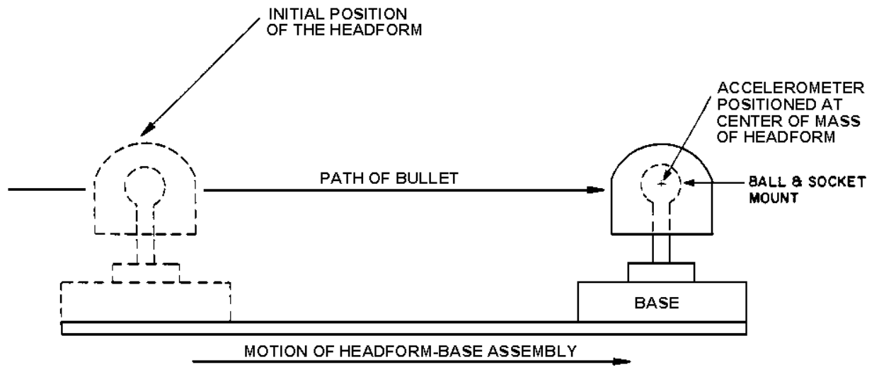
Figure 5. Ballistic impact test headform---base assembly.
