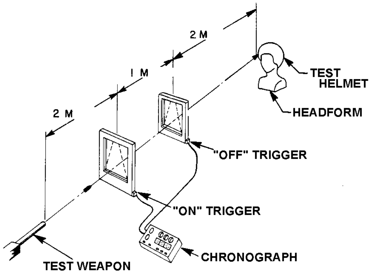
Figure 6. Test setup.
