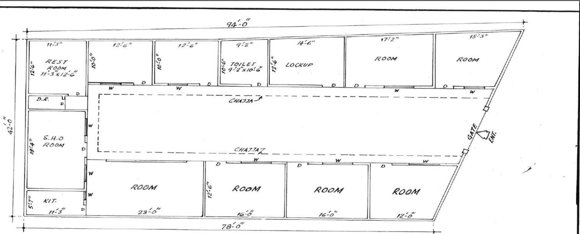
POLICE STATION PLAN
